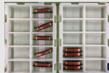
Reflectone single-coil pickup after the coil winding process
